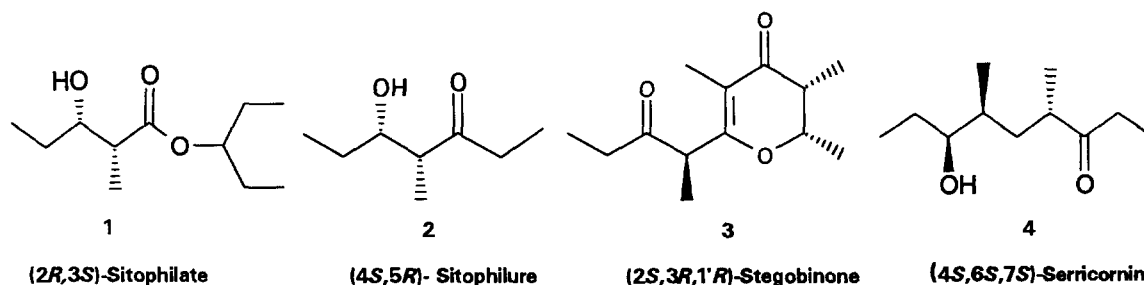
Figure 1. Structures of compounds 1 , 2 , 3 and 4 .
